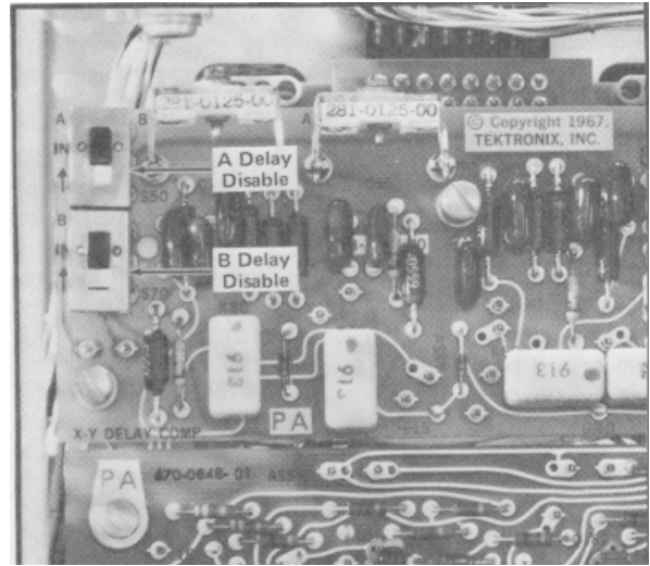
Fig. 2-6. Location of A and B Delay Disable
