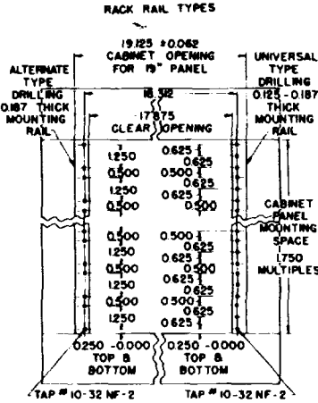
Fig. 6-7. Dimensional drawing of R7704.
